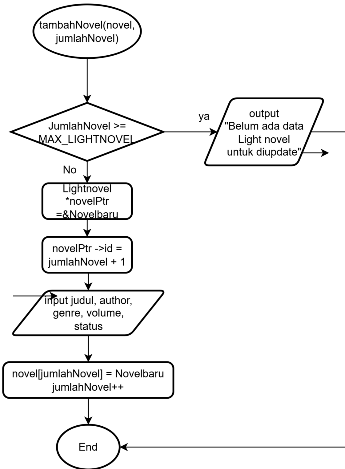
Gambar 1.5 Flowchart Create(tambahNovel)
